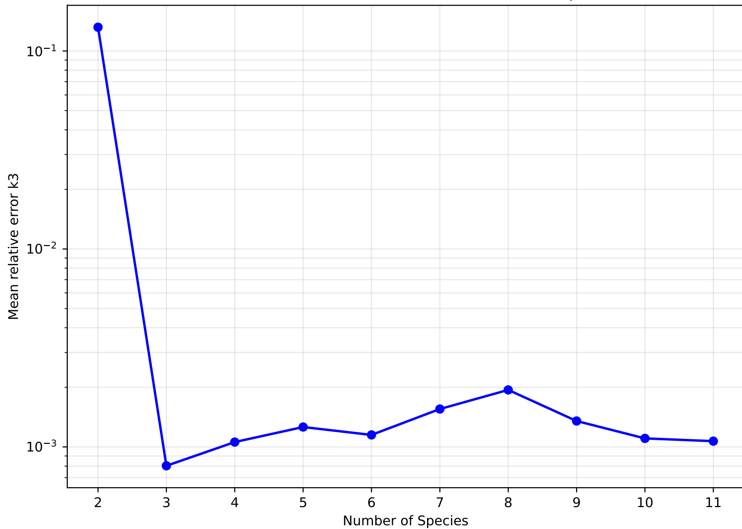
30, 30 — Mean relative error k3 vs number of species
